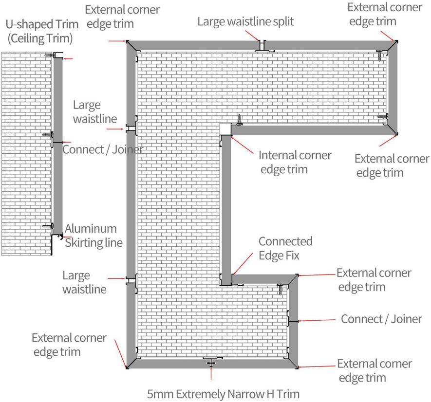
Hidden Door Installation Detail Drawing
