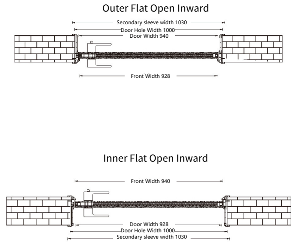
Model 25 Installation Diagram
